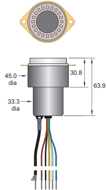
B19A socket with optional flange shown dashed
